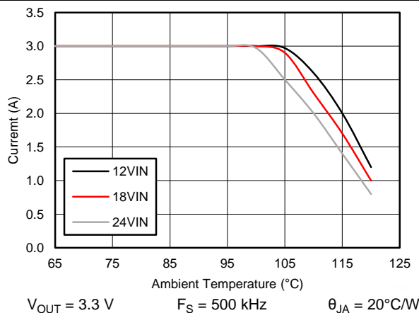
Figure 66. Derating Curve
