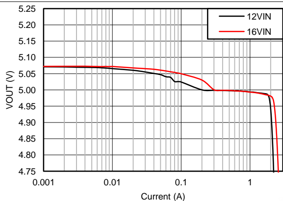
V_{OUT} = 5\text{ V} F_S = 2.2\text{ MHz}
