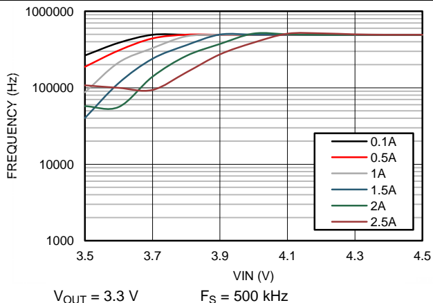
Figure 62. Frequency vs VIN
