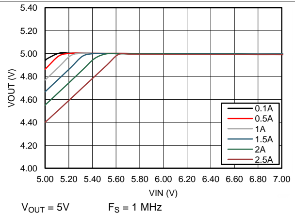
Figure 16. Dropout Curve
