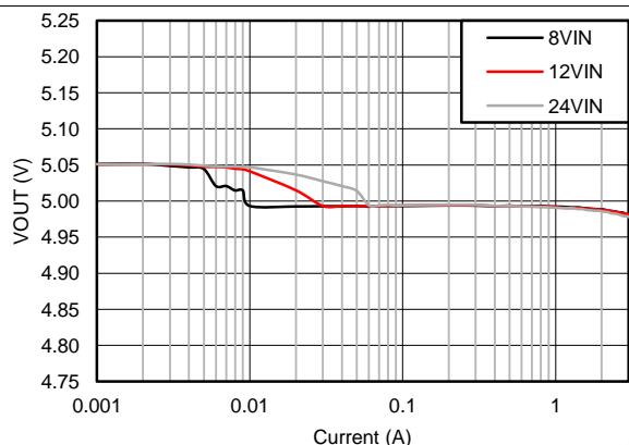
V_{OUT} = 5\text{ V} F_S = 500\text{ kHz}
