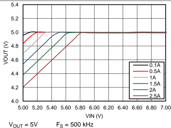
Figure 15. Dropout Curve
