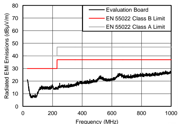
LM43603PWPEVM Radiated Emission Graph 12V IN to 3.3V OUT , F S = 500 kHz, I OUT = 3A
