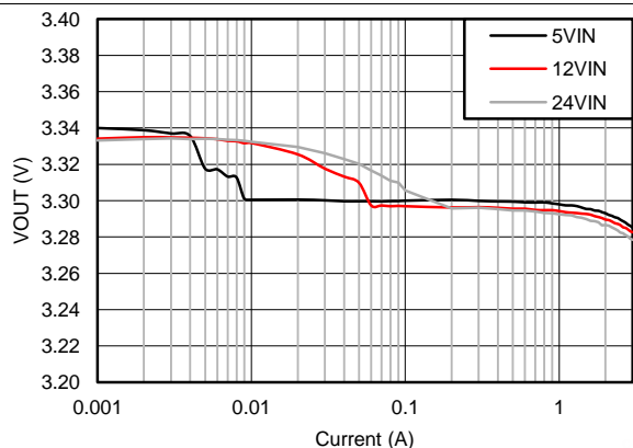
V_{OUT} = 3.3\text{ V} F_S = 500\text{ kHz}
